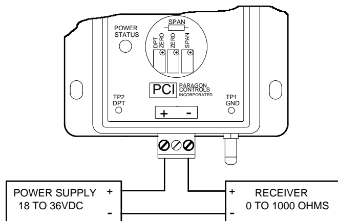
ELECTRICAL CONNECTIONS
