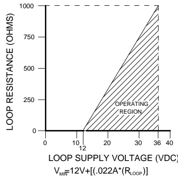
4-20mA LOAD LIMITATIONS
